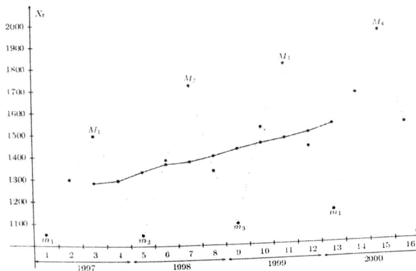
FIGURE 3.5 – Tendence - Moyennes mobiles centrées, k = 4 = 2 \times 2
