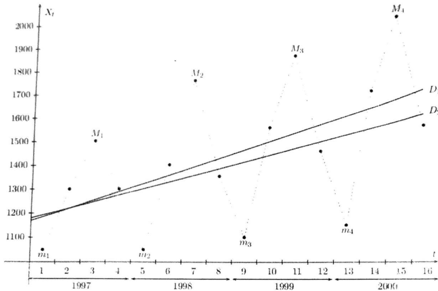
FIGURE 3.3 – Tendance - Ajustement linéaire
